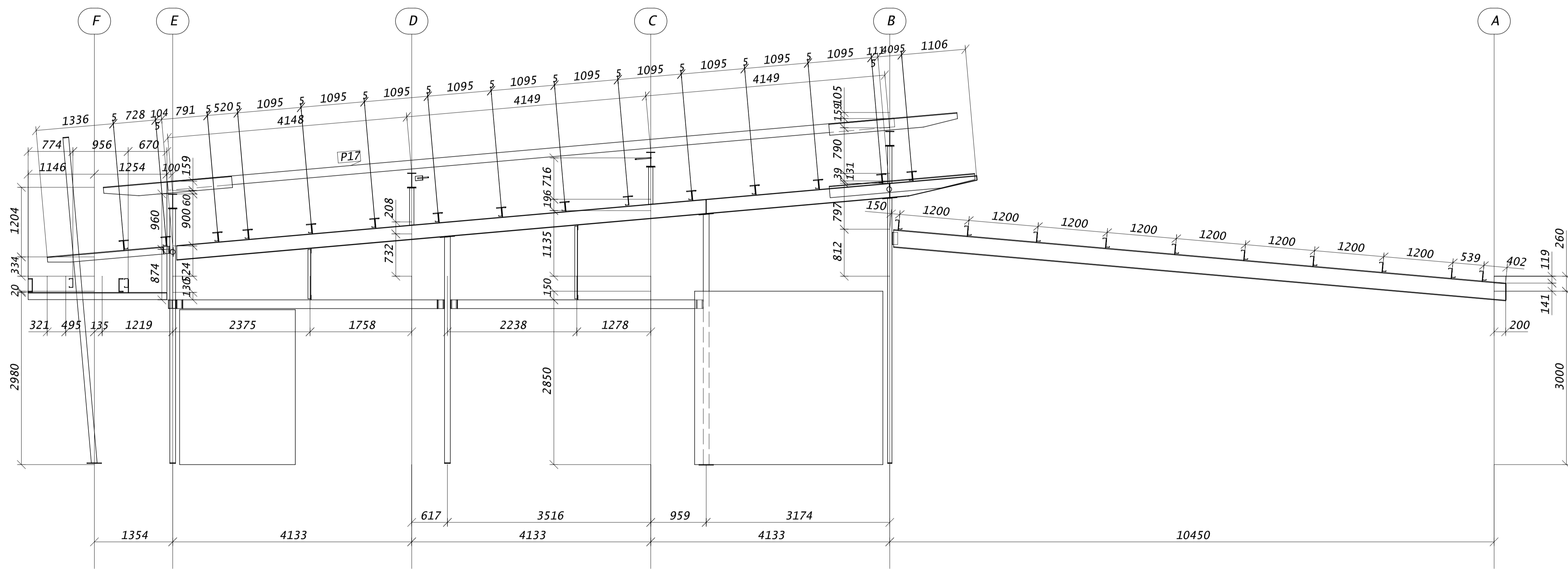
ELEVATION ABOUT GRINDLINE 5
